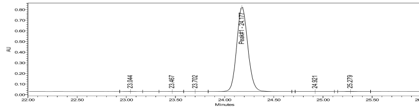
HPLC-UV Chromatogram
