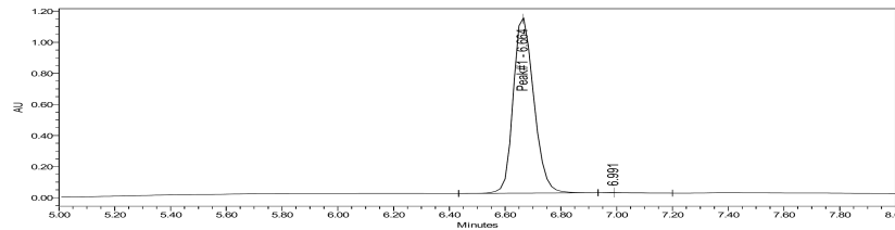
HPLC-UV Chromatogram
