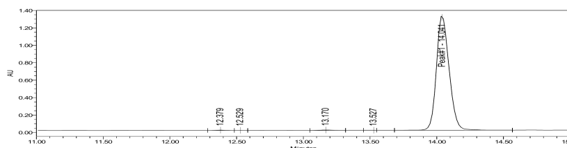
HPLC-UV Chromatogram
