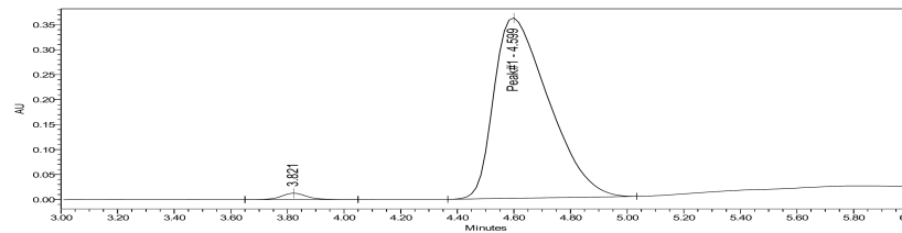
HPLC-UV Chromatogram
